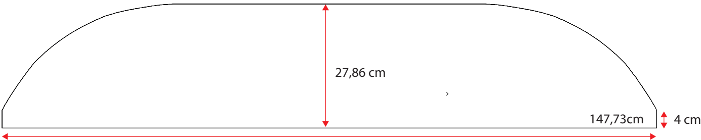
481004128 Wheel arch cover. Double Tabbert 2017
